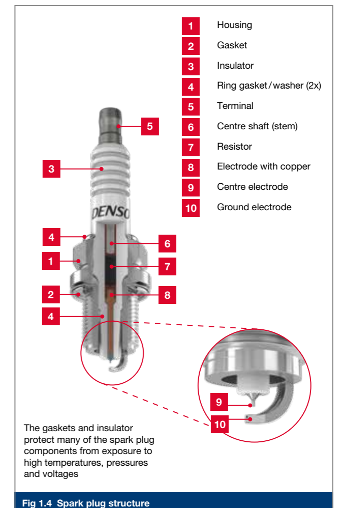
Fig 1.4 Spark plug structure
