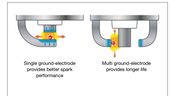
Fig 10.4 Performance of single electrode compared to side electrodes
