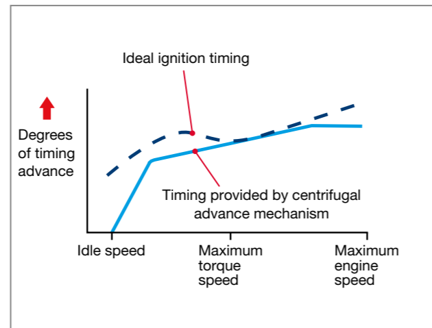
Fig 4.6 Limitations of centrifugal advance mechanism
