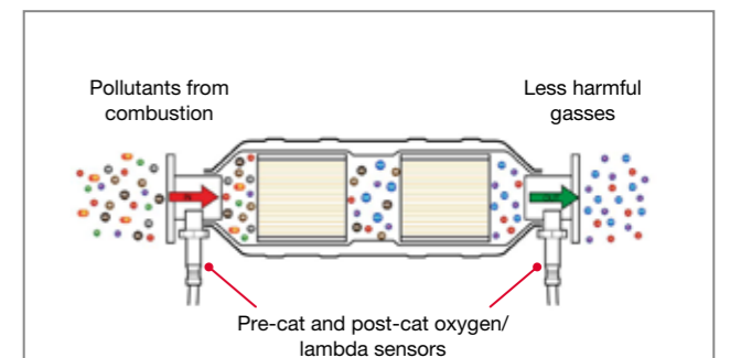
Fig 5.12 Catalytic converter
