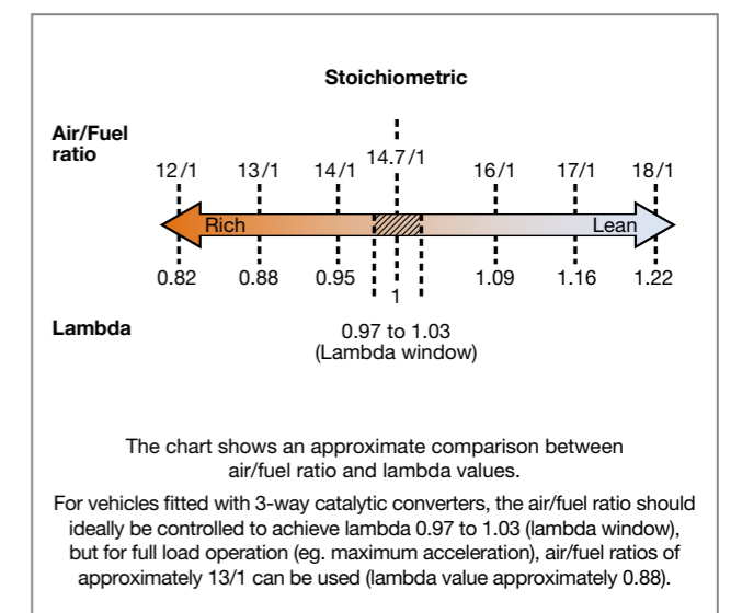
Fig 5.4 Air/fuel ratio compared to lambda
