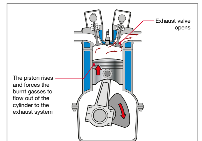
Fig 2.4 Exhaust stroke
