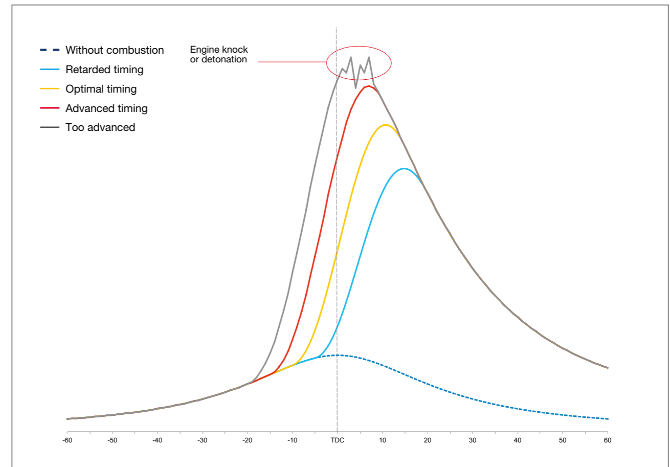
Fig 3.13 Comparison of advanced, retarded and optimal ignition timing
