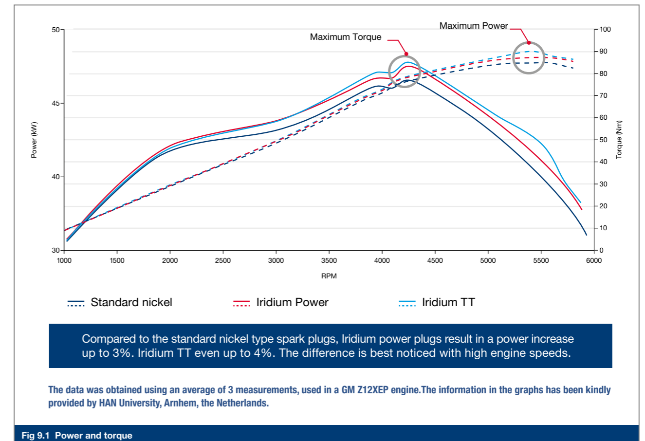
Fig 9.1 Power and torque
