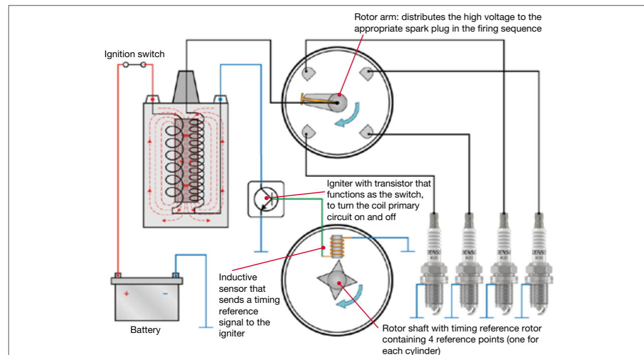
Fig 4.9 Basic electronic ignition system
