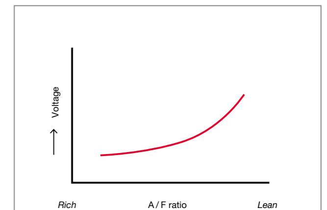
Fig 6.9 Voltage required to create a spark is higher with leaner air/fuel ratios
