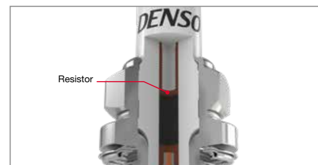
Fig 7.15 Resistor plug
