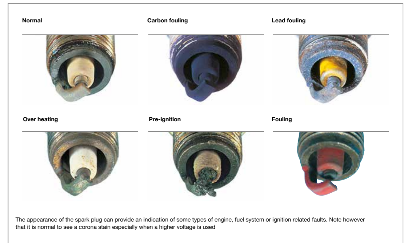
Fig 10.6 Diagnosis faults using spark plug appearance
