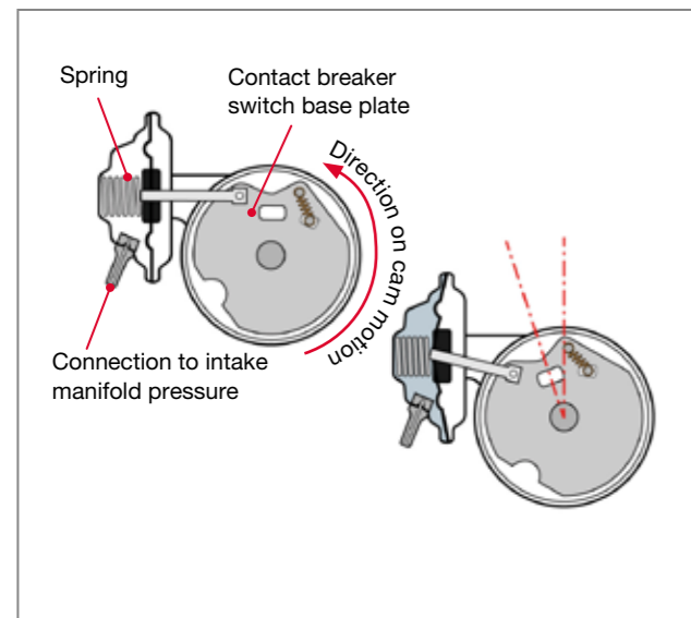
Fig 4.5 Engine load related mechanical timing advance
