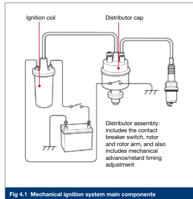
Fig 4.1 Mechanical ignition system main components
