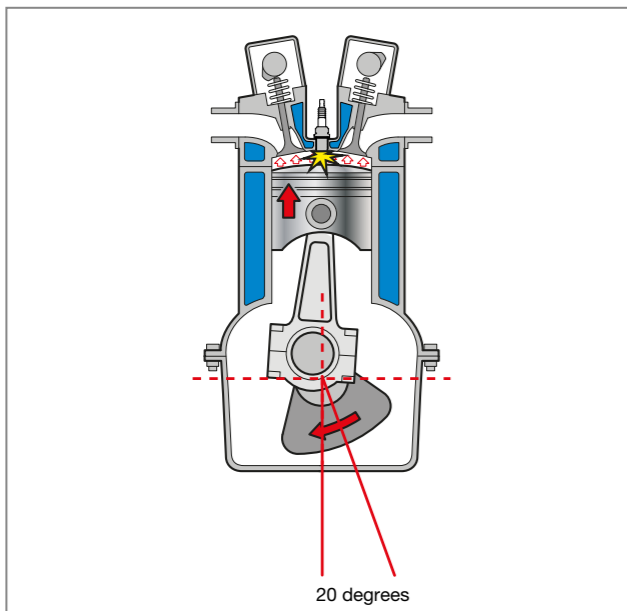
Fig 3.8 Ignition timing occurring at 20 degrees before Top Dead Centre (TDC)
