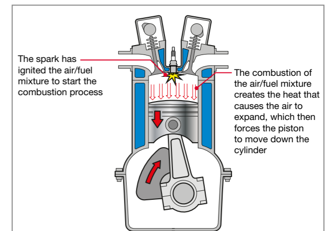
Fig 2.3 Ignition/power stroke
