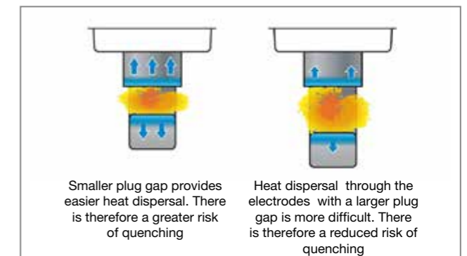
Fig 6.16 Quenching effect created by small and large plug gaps
