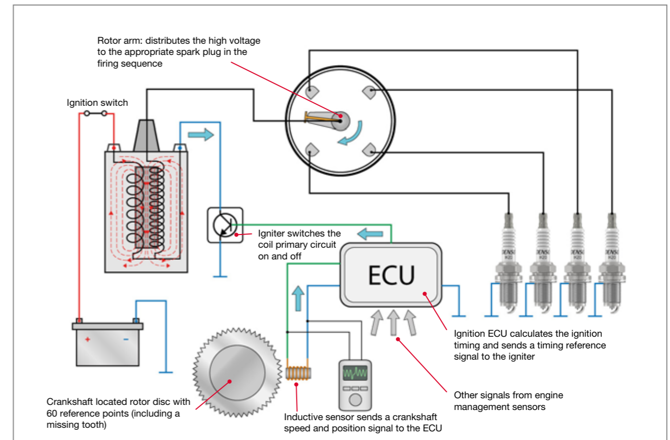
Fig 4.10 Distributorless electronic ignition system controlled by engine management ECU
