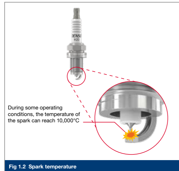
Fig 1.2 Spark temperature
