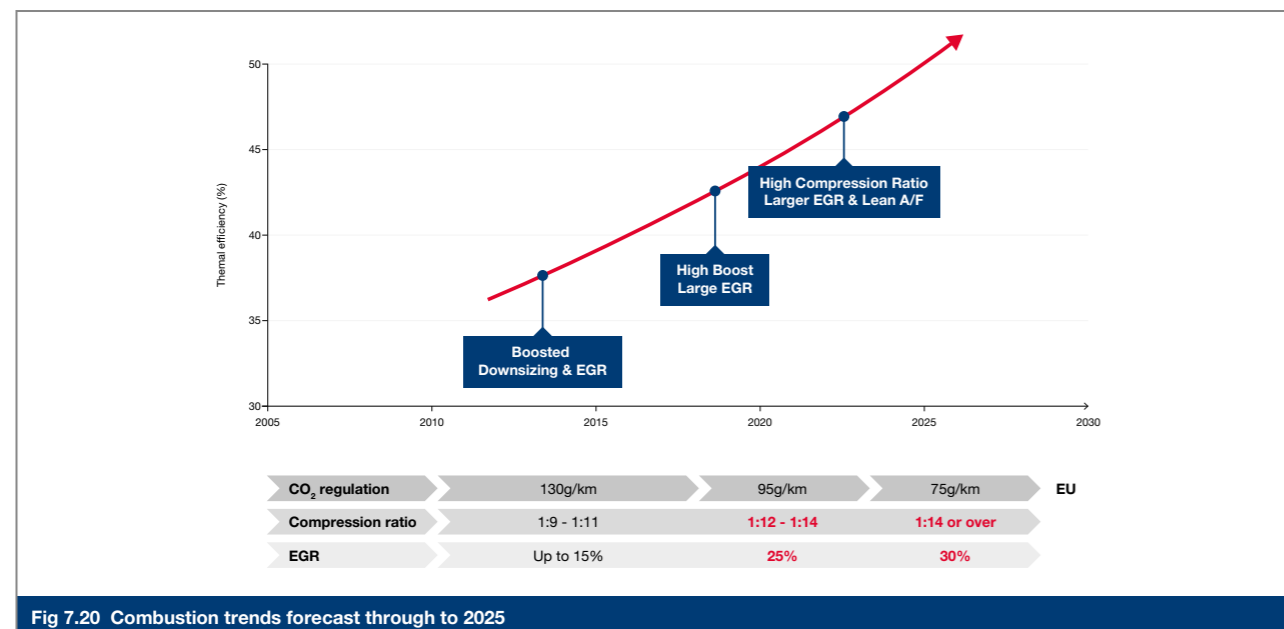
Fig 7.20 Combustion trends forecast through to 2025
