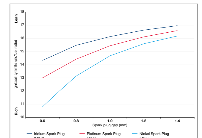
Fig 7.23 Comparison of ignitability limits with different spark plug gaps for different spark plug types
