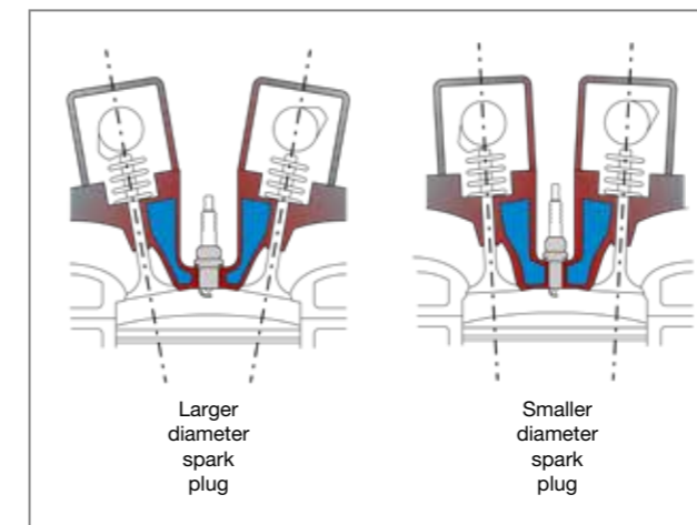
Fig 7.21 Narrower spark plug with longer thread occupying less space on the cylinder head
