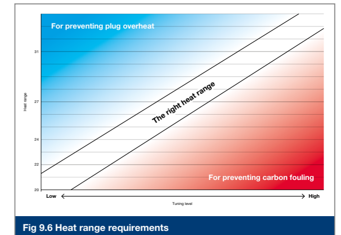
Fig 9.6 Heat range requirements
