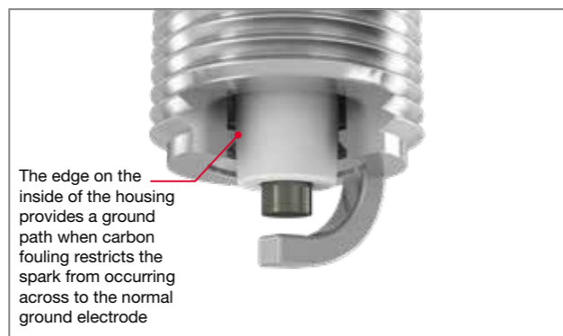
Fig 7.11 Semi-surface gap
