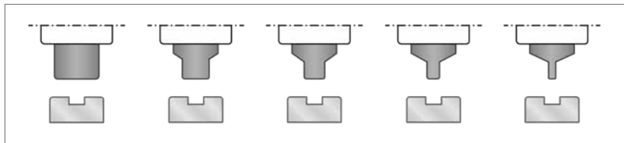
Fig 7.3 Examples of different types and sizes of centre electrodes
