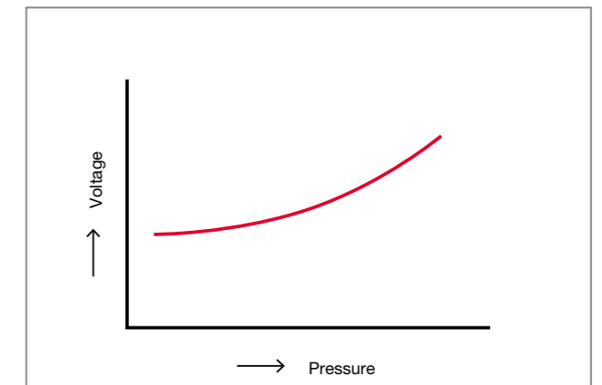
Fig 6.8 Voltage required to create a spark is higher with the increase in compression pressure
