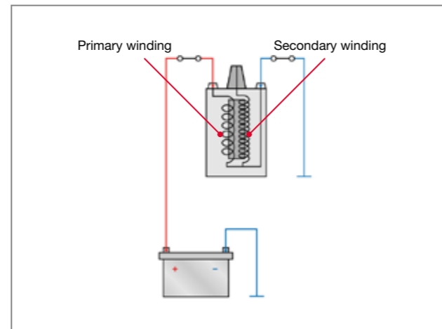
The secondary winding in an ignition coil has more windings than the primary winding. When the magnetic field collapses, the voltage induced in the secondary will be greater than in the voltage induced in primary winding.
