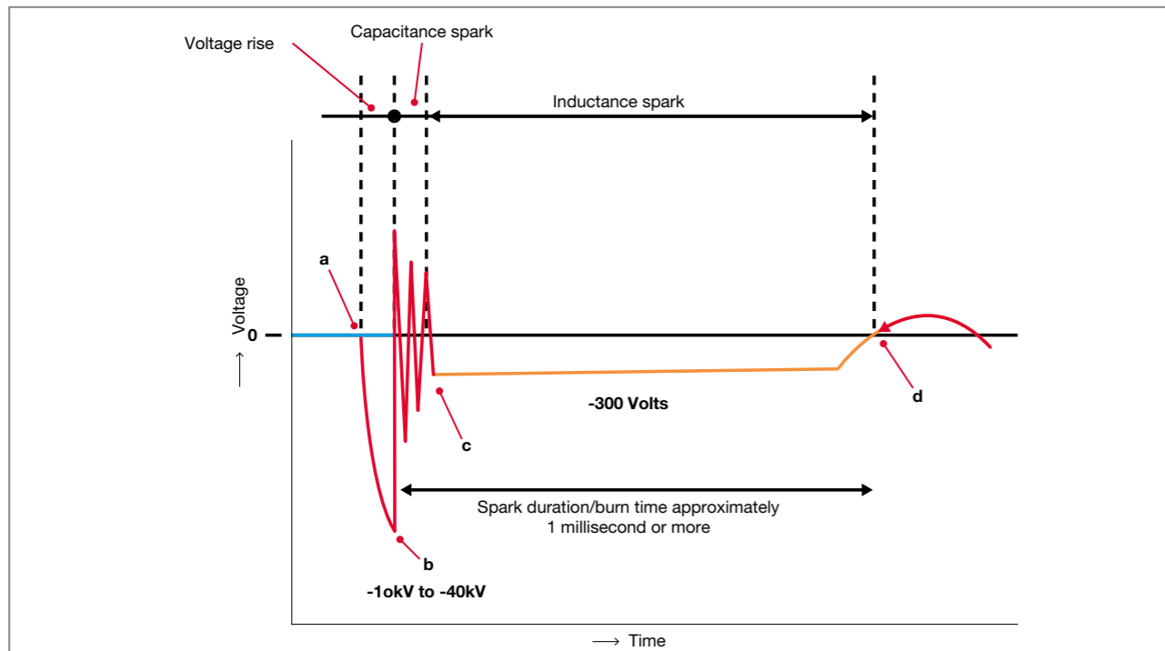
Fig 6.4 Different phases and voltages when the spark is generated and maintained
