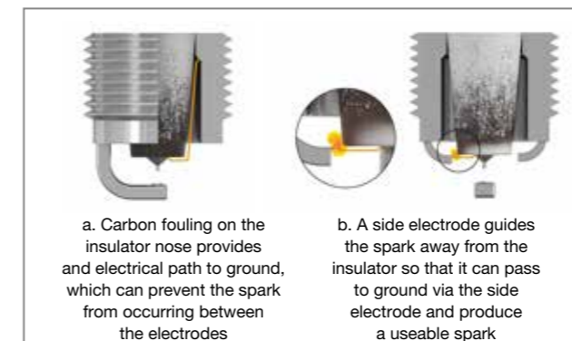
Fig 10.3 Benefit of side electrodes
