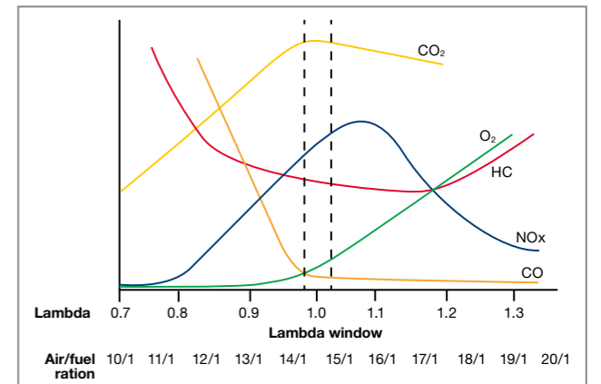
Fig 5.11 Air/fuel ratio affecting pollutant levels
