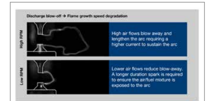
Fig 7.22 Combustion air flow affecting spark blow-away
