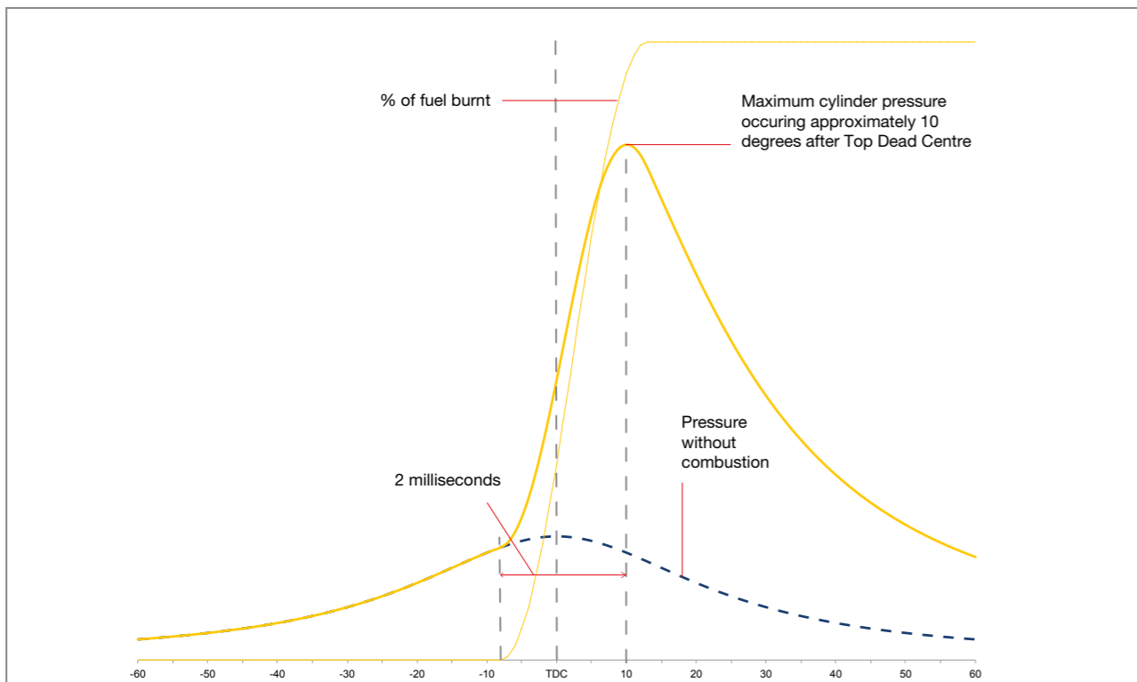
Fig 3.9 Setting ignition timing approximately 2 milliseconds before maximum cylinder pressure is required
