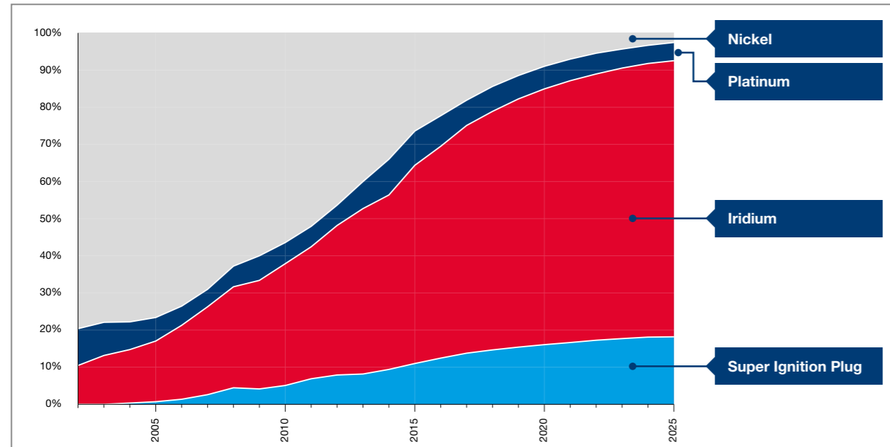
Fig 7.19 Market share for different spark plug types (forecast through to 2025)
