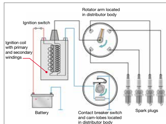
Fig 3.1 The main components of a Kettering type ignition system
