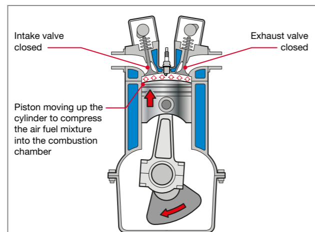
Fig 2.2 Compression stroke
