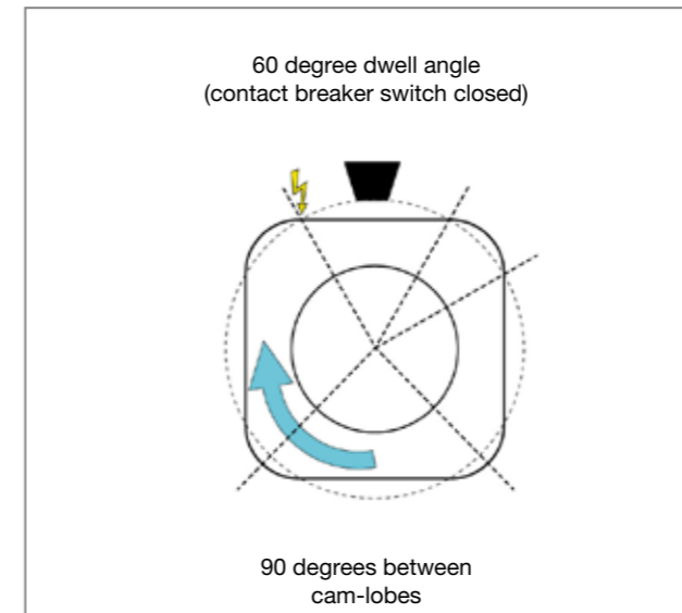
Fig 4.7 Dwell angle shown as 60 degrees of distributor shaft rotation
