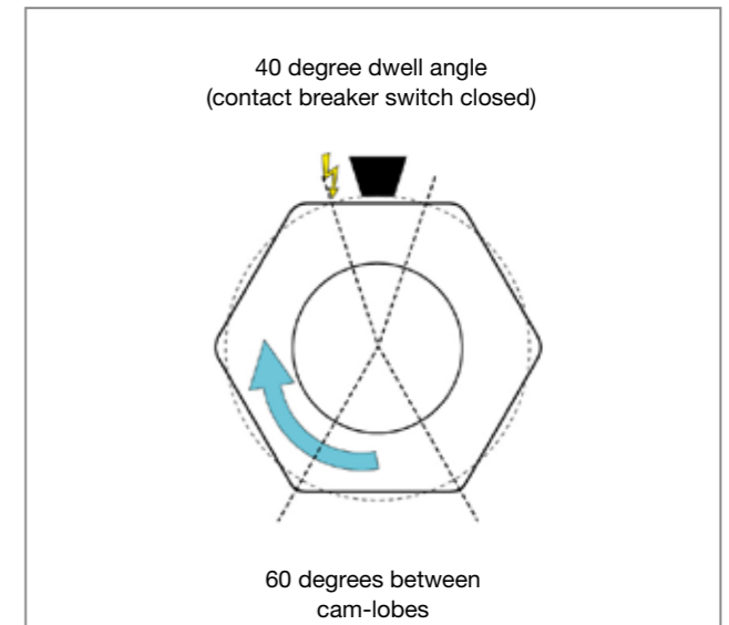
Fig 4.8 Dwell angle shown as 40 degrees of distributor shaft rotation for a 6-cylinder engine
