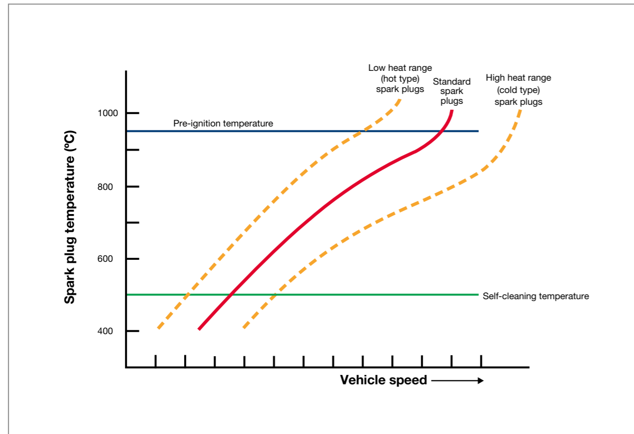
Fig 6.14 Different vehicles speeds affecting the critical spark plug temperatures for spark plugs with different heat ranges
