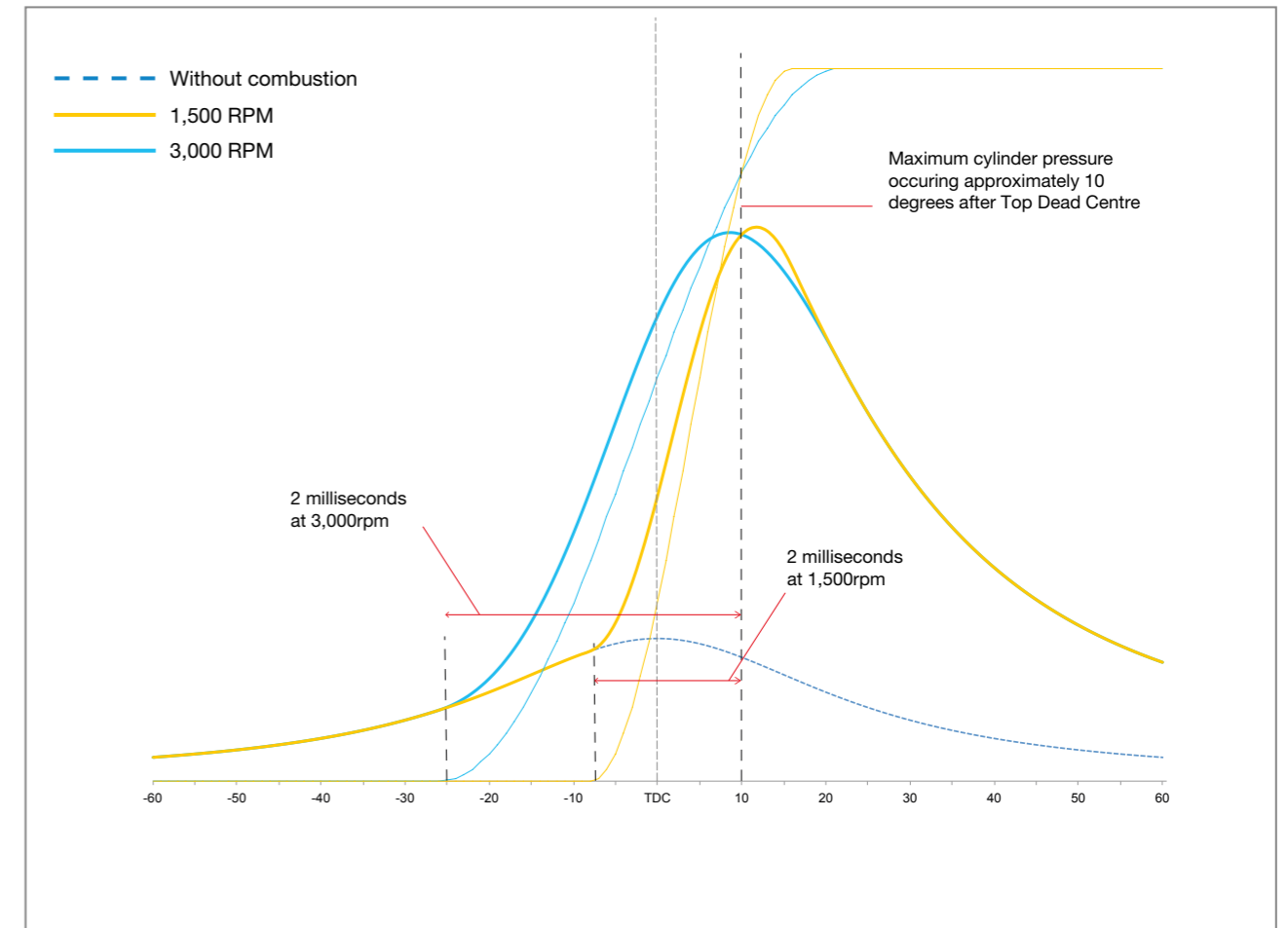
Fig 3.10 Ignition timing advance at 1,500 and 3,000rpm
