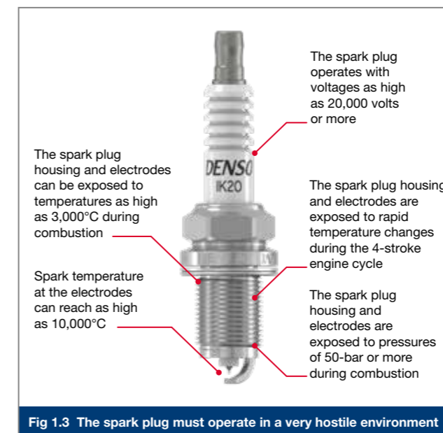
Fig 1.3 The spark plug must operate in a very hostile environment
