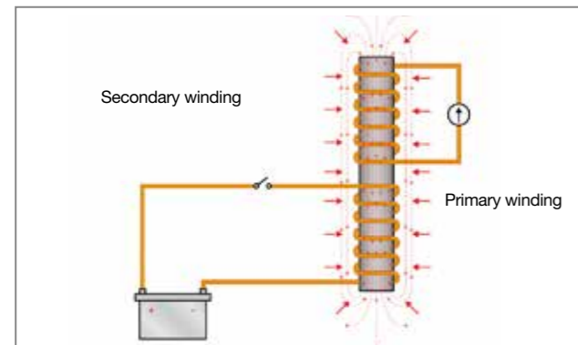
The magnetic field in the primary winding also surrounds the adjacent secondary winding. Collapsing the field induces electric currents in both windings.
