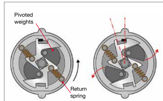
Fig 4.4 Speed related mechanical timing advance mechanism
