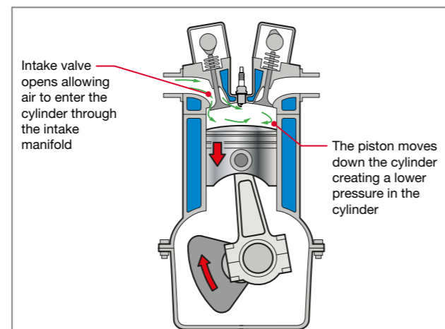
Fig 2.1 Intake stroke
