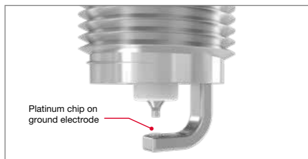
Fig 7.13 Platinum chip ground electrode
